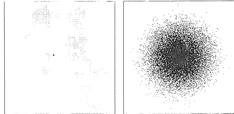
Figure 15.1: (a) Tangled path of a particle in a two-dimensional random walk (magnified view). (b) Gradual diffusion of a dense cluster of particles.
