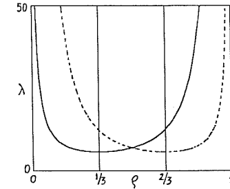
Figure 15.5: The solid line plots the mean free path \lambda as a function of the particle density \rho , in TM-GAS; the dashed curve plots the mean free path for the “holes.”
