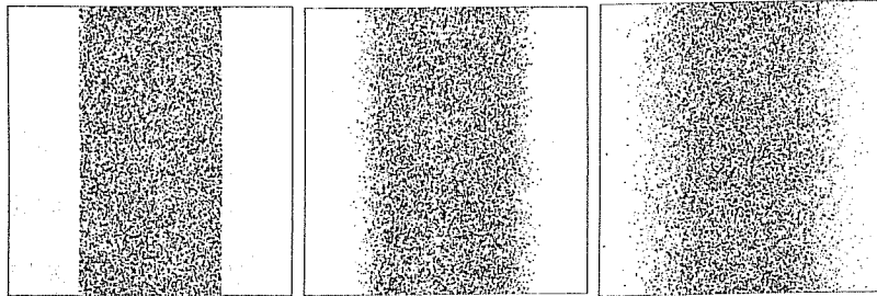
Figure 15.4: Self diffusion of two gases having different colors but identical dynamical properties.
