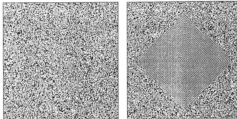
Figure 9.8: (a) Typical contour levels for the phase "sheet." In (b), the sheet has been "nailed down" at one spot by permanently deactivating one cell's clock.
