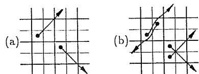
Figure 12.2: SWAP-ON-DIAG: (a) Uniform motion of a particle (here and in the following figures the particle is shown at the beginning of an even step—where the relevant blocks are those delimited by thick lines). (b) Particles go “through” one another without interacting.
