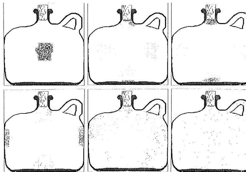
Figure 15.3: Expansion of a TM-GAS cloud in a vacuum. Repeated collisions between particles and with container's walls eventually lead to thorough thermalization.
