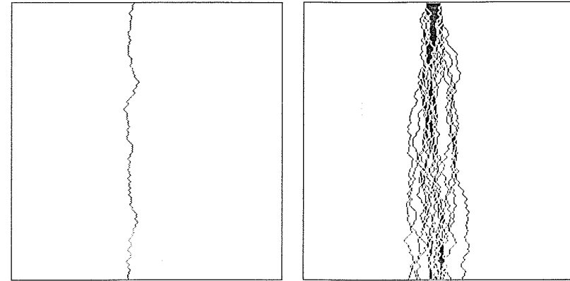
Figure 10.1: Random walk: (a) Spacetime history of a one-particle system, using the “left/right” approach. (b) A many-particle system, using the “swap” approach.
