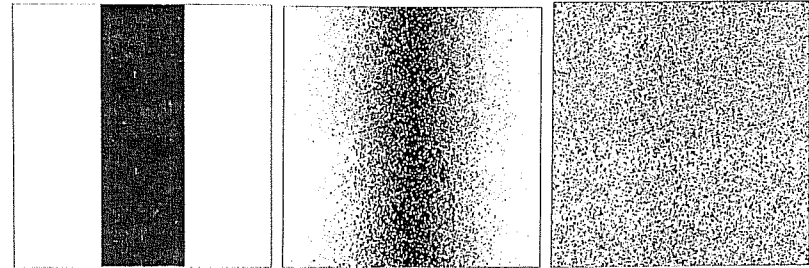
Figure 10.2: Initially separated (a), ink and water diffuse into each other (b), eventually producing a uniform mixture (c).
