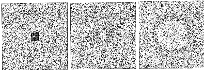
Figure 16.4: Wave propagation in a denser realization of the HPP gas model. To enhance contrast, only sites that contain three or four particles are shown.
