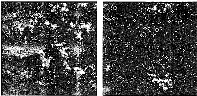
Figure 3.2: (a) Hundreds of steps later activity is concentrated in a few smoldering areas, with occasional flares. (b) A few thousand steps later, most action has died out.
