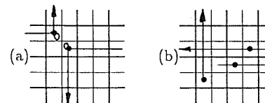
Figure 12.5: TM-GAS (a) Particles that collide within a block bounce at a 90° angle; the little loop is a reminder that they stay in the same place for one step. (b) Collisions do not occur for particles that fly past one another on adjacent blocks, or for particles that travel orthogonally.
