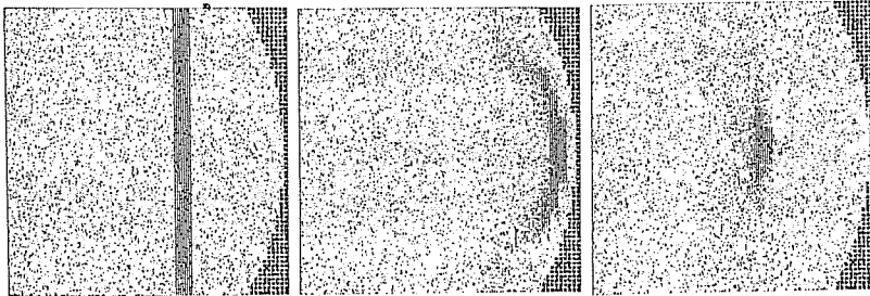
Figure 16.7: A plane pulse traveling towards a concave mirror (a) is shown right after the reflection (b) and approaching the focal point (c).
