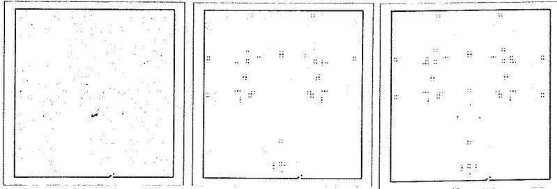
Figure 18.9: Magic-gas experiment: (a) A gas; (b) something happening; and (c) order out of disorder.
