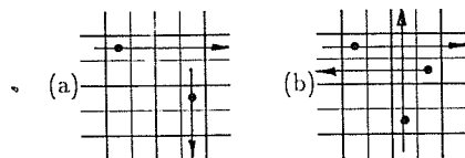
Figure 12.4: ROT-CW/CCW: (a) Uniform motion of a particle. (b) Particles pass by one another without interacting.
