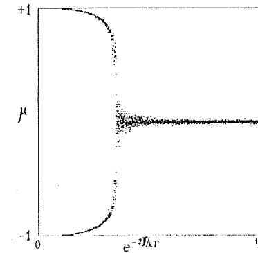
Figure 17.6: Magnetization \mu in the canonical-ensemble model, versus the Monte Carlo acceptance probability. Note the sharp transition at the critical temperature T_{\text{crit}} .
