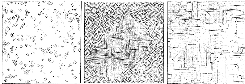
Figure 6.2: GREENBERG: Initial, intermediate, and steady-state behavior, starting with 3% of 1's at random in one plane and a different 3% random pattern in the other.
