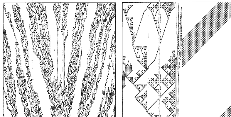
Figure 4.1: Behavior of HGLASS (a) from random conditions and (b) from a simple seed.
