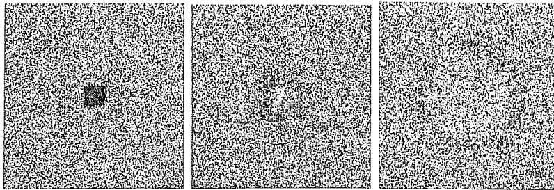
Figure 16.1: Circular wave produced by a localized disturbance.
