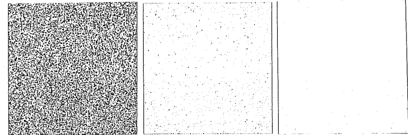
Figure 8.1: Exponential decay driven by a random source.
