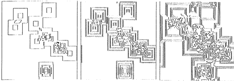
Figure 11.1: Successive stages of the BORDER/HOLLOW rule.
