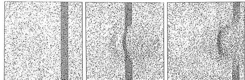
Figure 16.8: Refraction and reflection patterns produced by a spherical lens.
