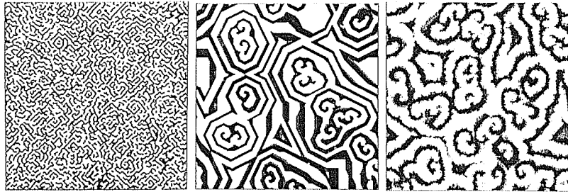
Figure 9.2: Spatial reactions: (a) and (b) use different values of a feedback parameter, while (c) is a non-monotonic threshold version of (b).
