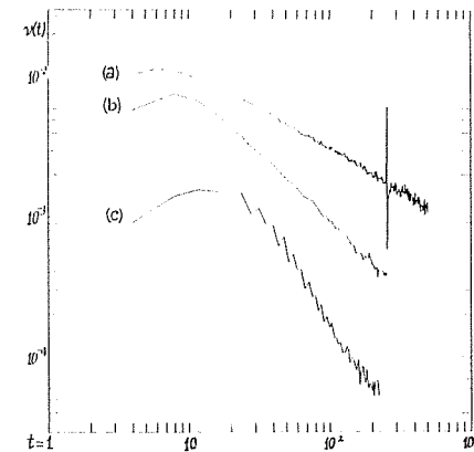
Figure 16.6: Time-correlation function \nu(t) for HPP-GAS (a), TM-GAS (b), and FHP-GAS (c).
