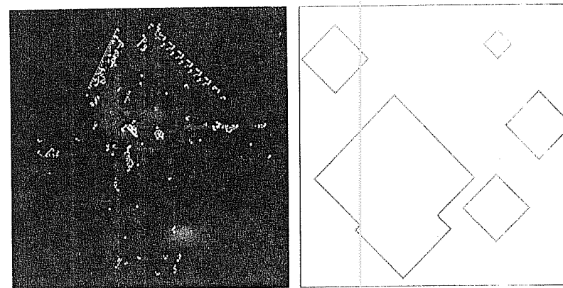
Figure 6.1: (a) Short time-exposure of BRIAN'S-BRAIN. (b) GREENBERG rule: isolated dots grow into rings, which merge into larger rings.
