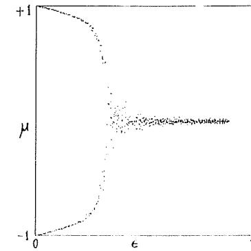
Figure 17.2: Magnetization \mu versus energy \epsilon . Below the critical value \epsilon_{\text{crit}} , two distinct values of \mu are possible.
